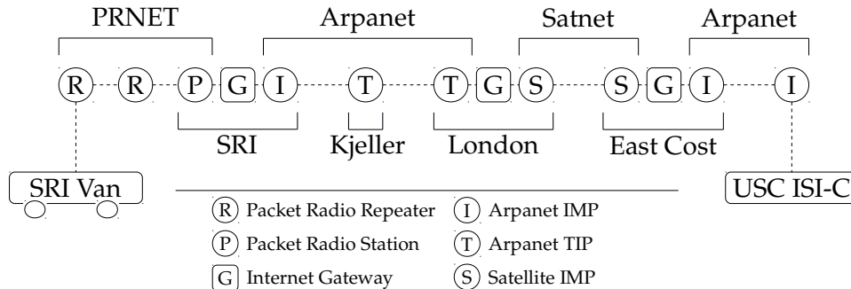
Figure N.8: First ARPA multinetwork TCP demonstration in November 1977; Source: Adapted from Kunzelman et al. (1978) as quoted in Nielson (2002, p. 5) (see also http://www.sri.com/about/timeline/images/1977map_000.jpg for a good quality diagram of the demonstration)
