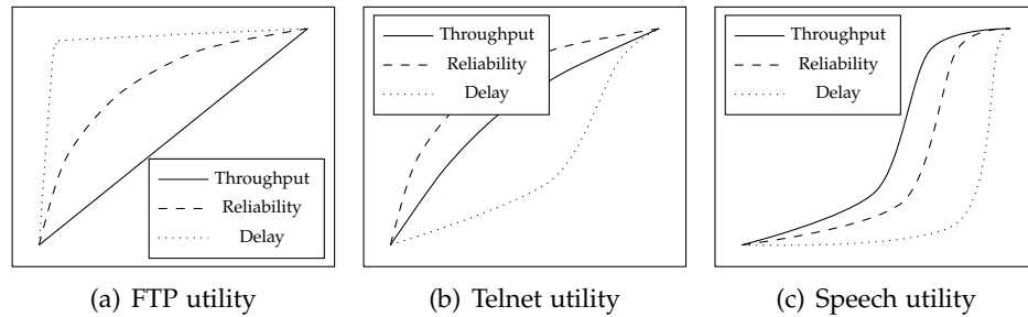
Figure 5.1: Utility of canonical application types as a function of throughput, reliability, and delay performance
